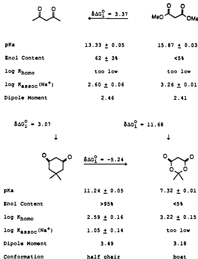
Figure 1. Comparison of various properties of cyclic and acyclic diketones and diesters with differences in standard free energies of ionization.
