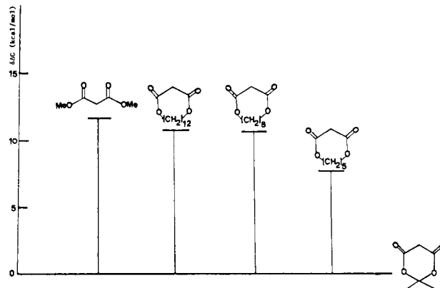
Figure 3. Effects of ring size on the acidities of cyclic \beta -Diesters.
